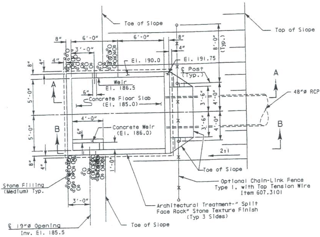
PLAN DR W-19 Scale: 1/4" = 1'-0"
